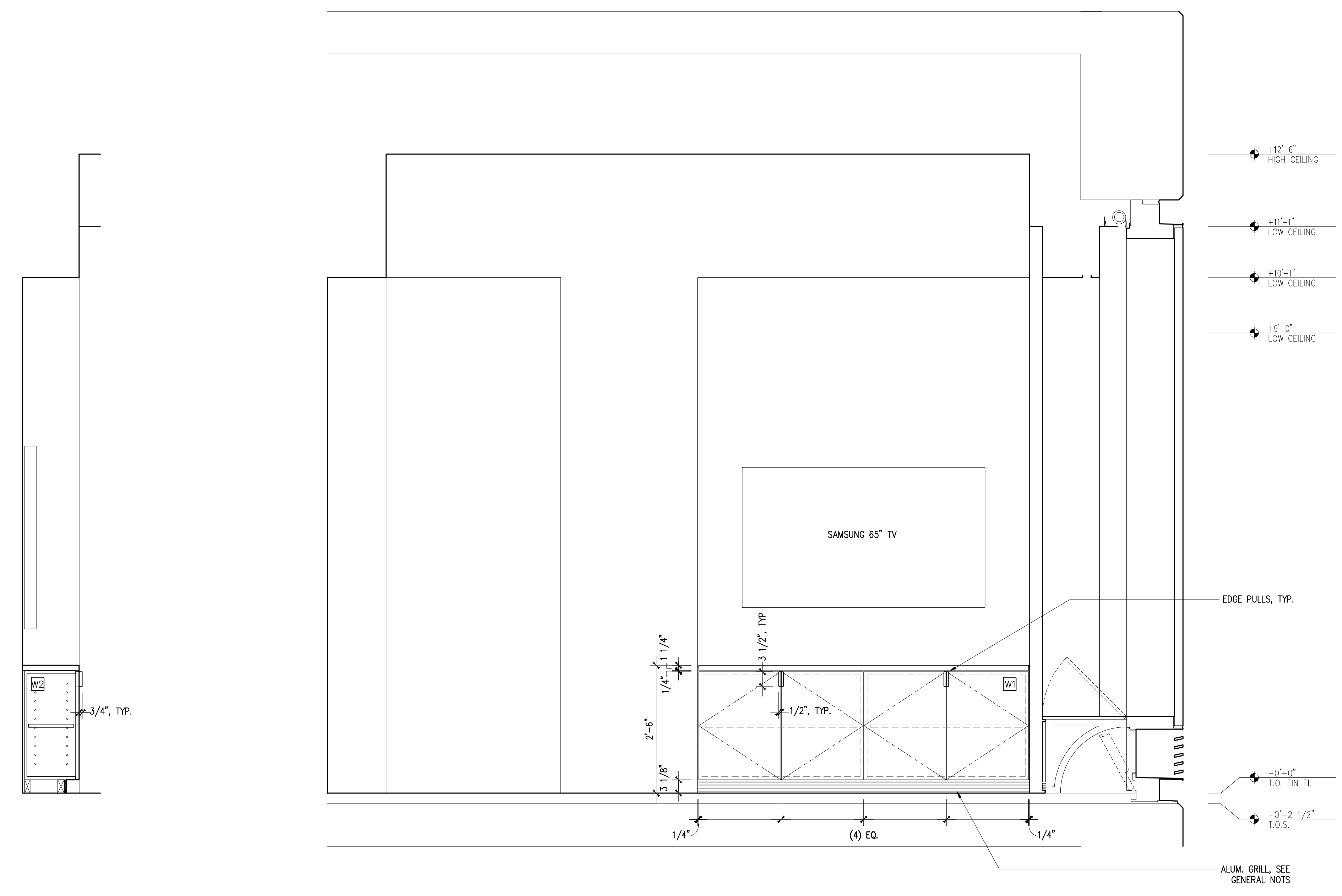
3 SECTION 3/4"=1'-0"
