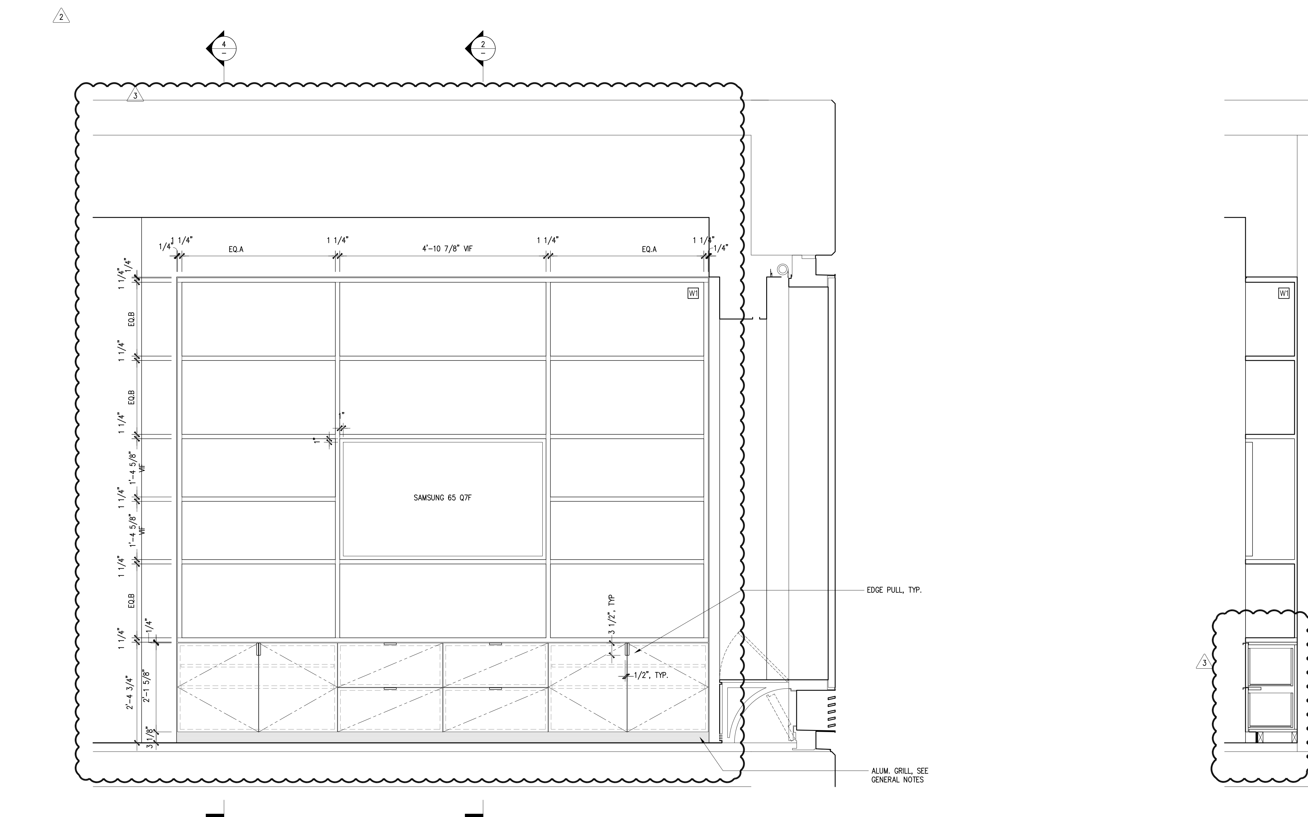
3 ELEVATION 3/4"=1'-0"
