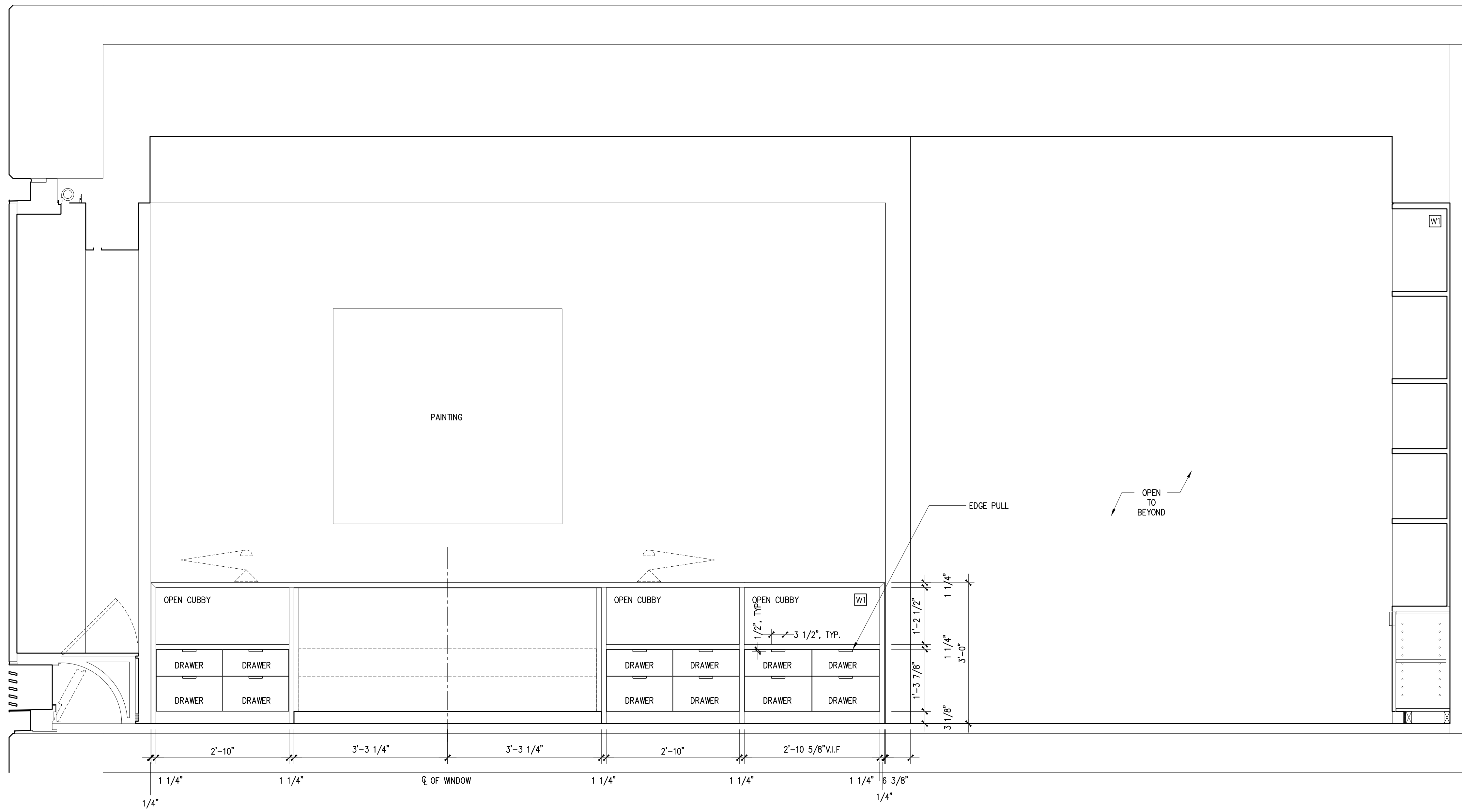
4 ELEVATION 3/4"=1'-0"
