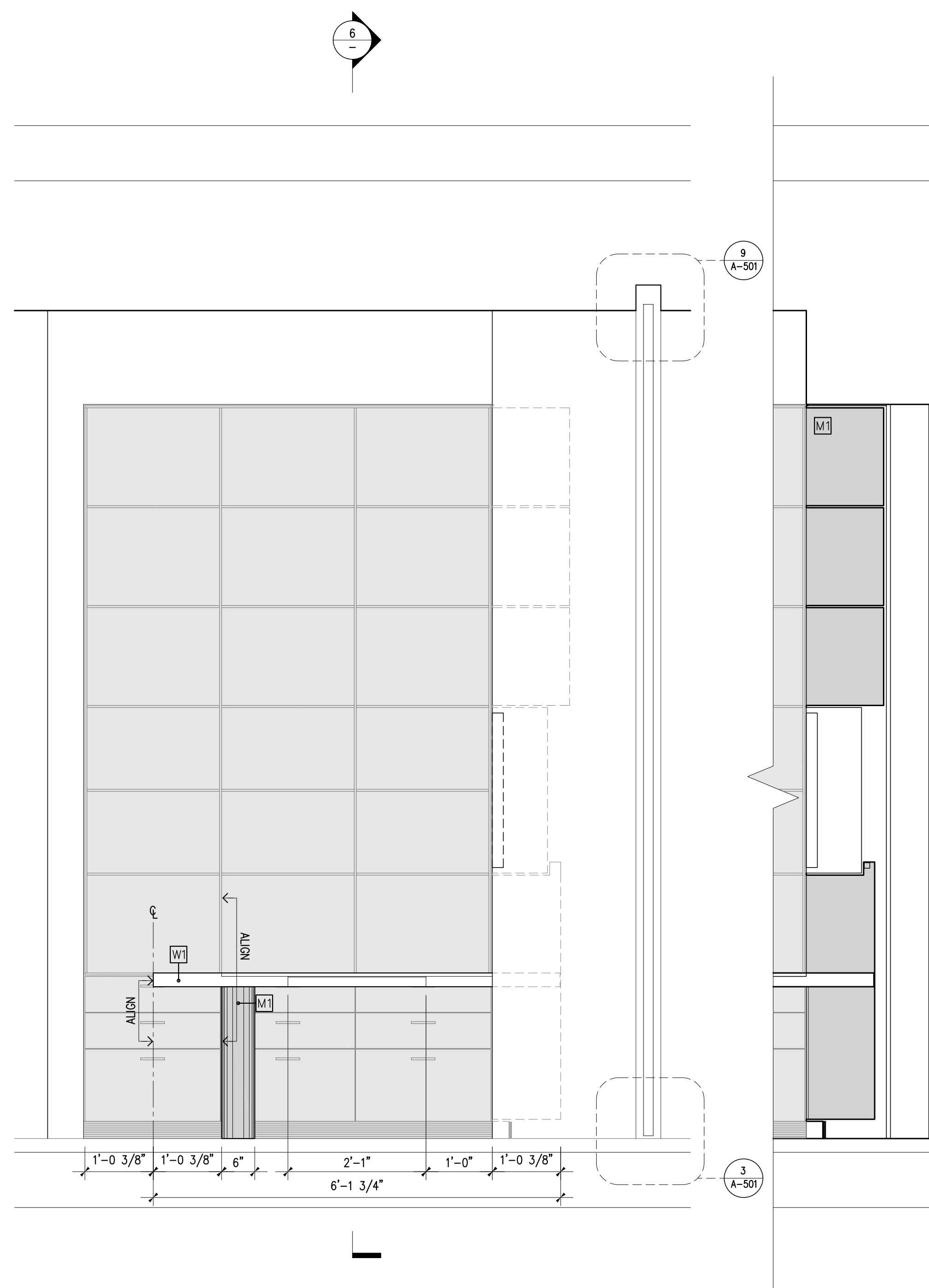
4 ELEVATION 3/4"=1'-0"
