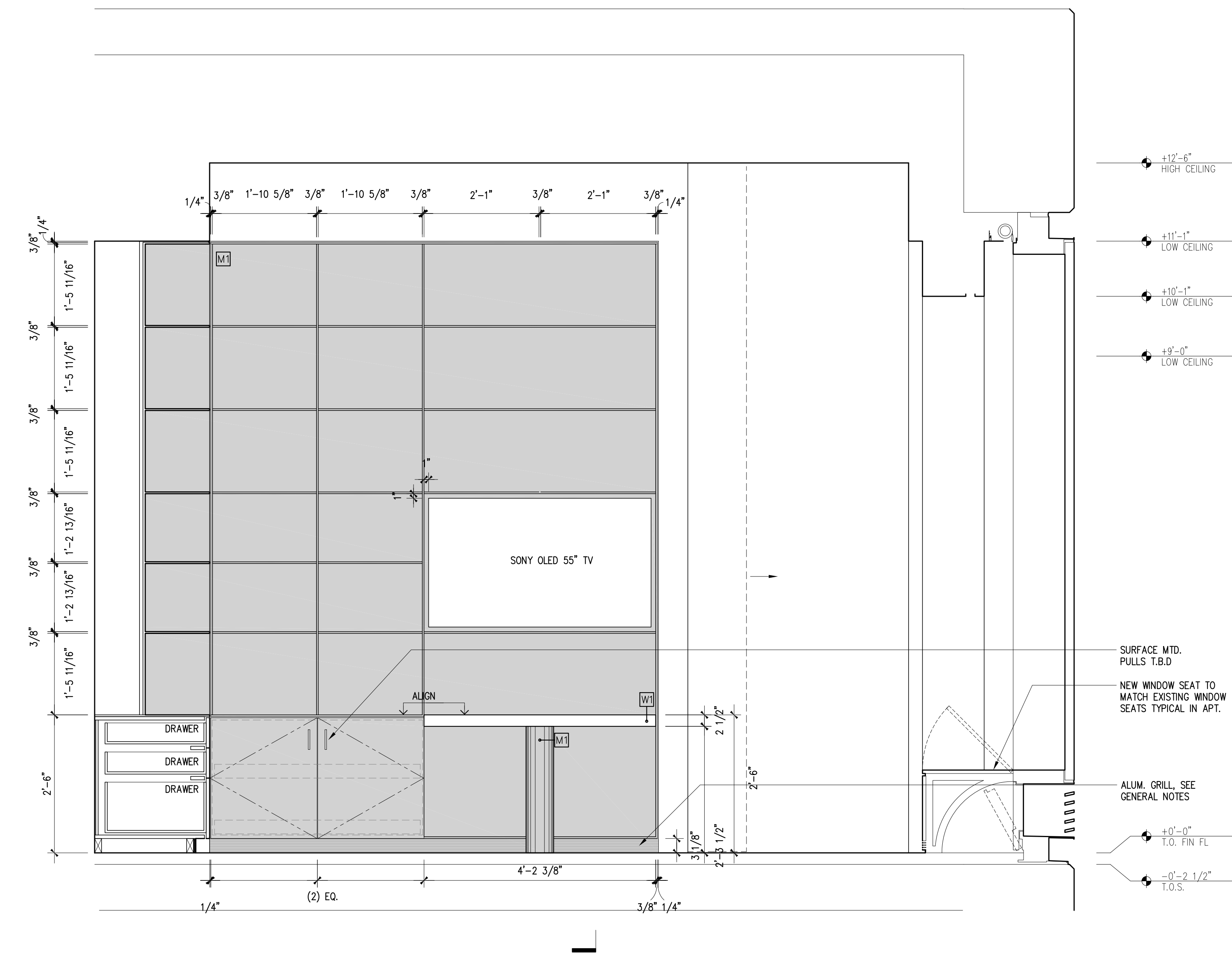
5 ELEVATION 3/4"=1'-0"
