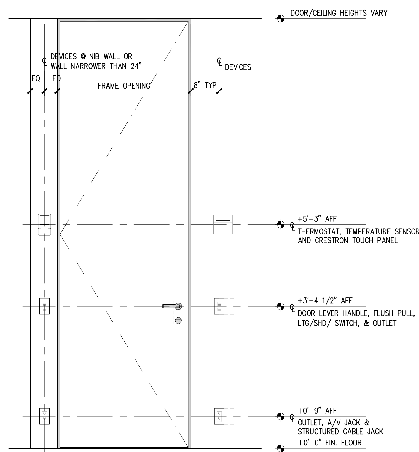
1 TYPICAL DEVICE LOCATIONS 3/4"=1'-0"
