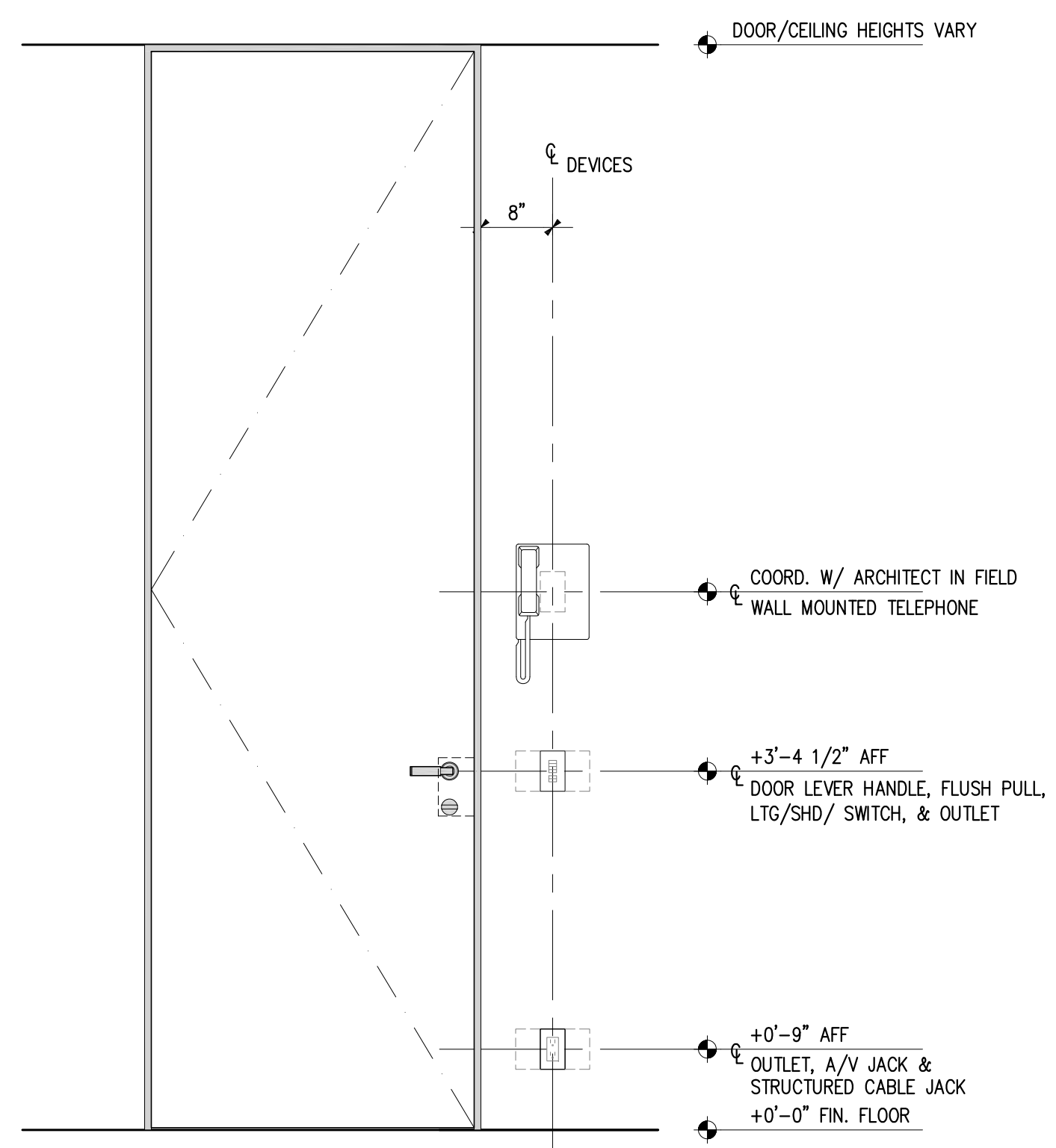
2 TYPICAL DEVICE LOCATIONS 3/4"=1'-0"
